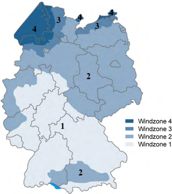
Windmap Germany
